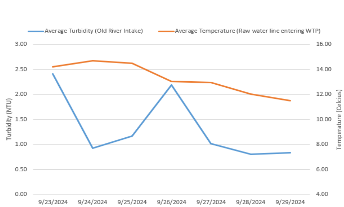
Englishman River Turbidity and Temperature
